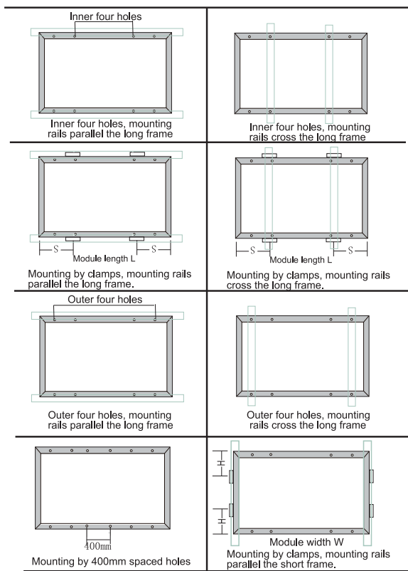
Figure 4 Installation Methods
