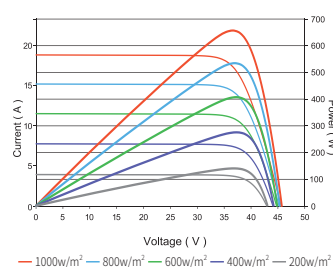
Current-Voltage & Power-Voltage Curves (665W)
