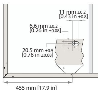
Fig. 9: Mounting holes: REC Alpha Panels
