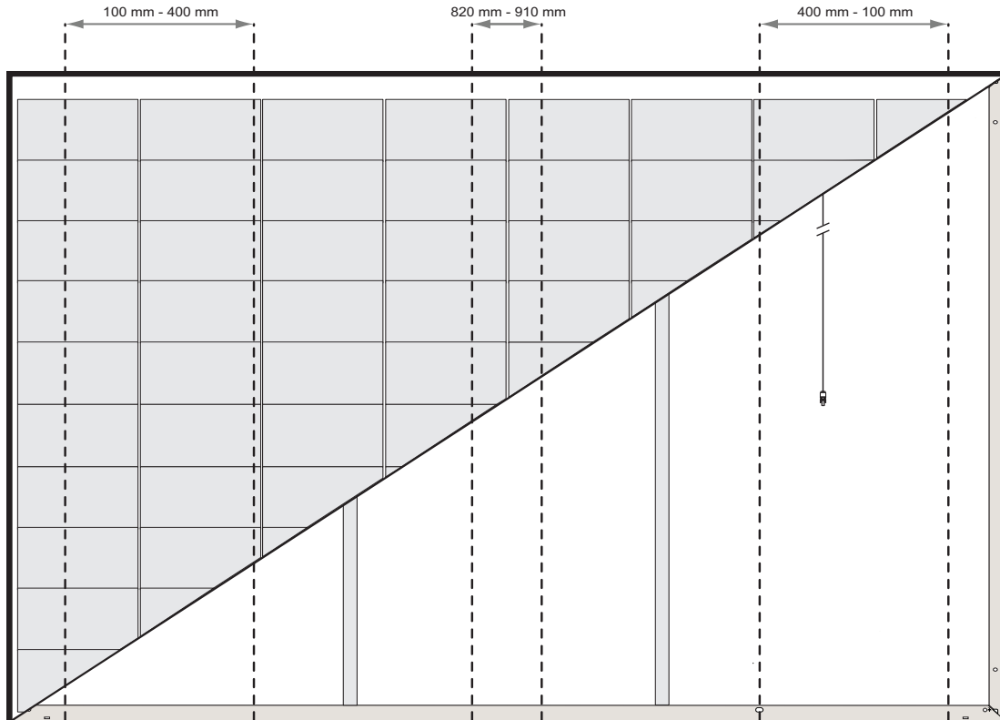
Fig. 13: Six-point mounting configuration clamping zones: REC Alpha Pure-R Series
