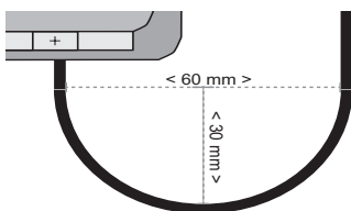
Fig. 15: Minimum cable bend radius
