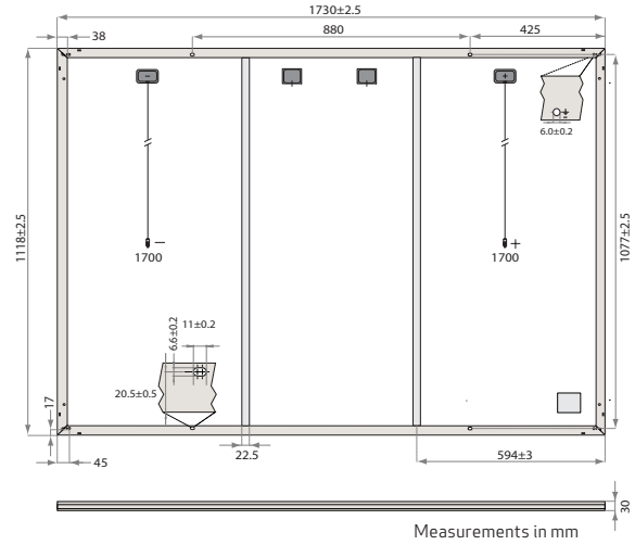
Fig. 18: Panel dimensions: REC Alpha Pure-R Series
