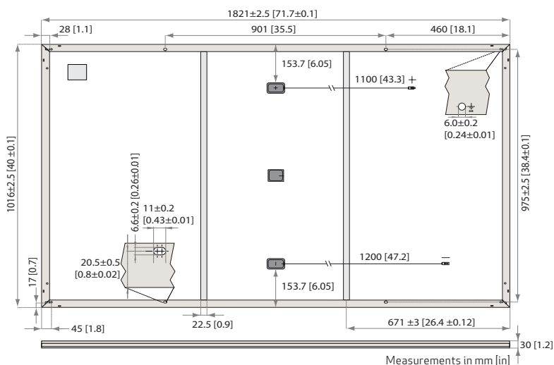
Fig. 17: Panel dimensions: REC Alpha Pure Series
