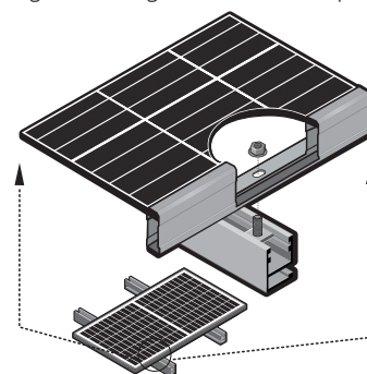
Fig. 11: Mounting hole installation example
