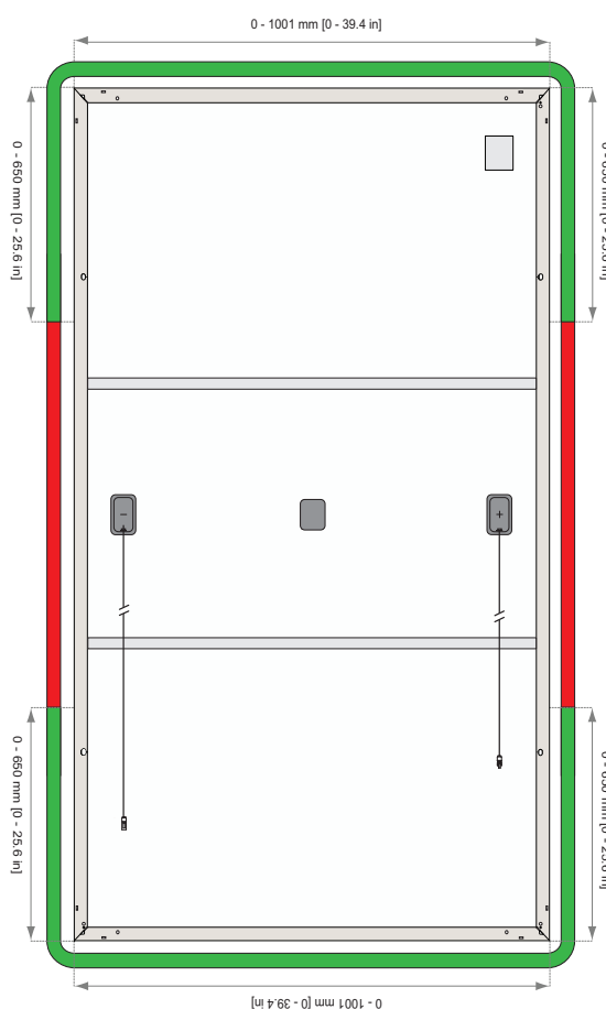
Fig. 27: REC 72-cell panels MLPE device installation zones
