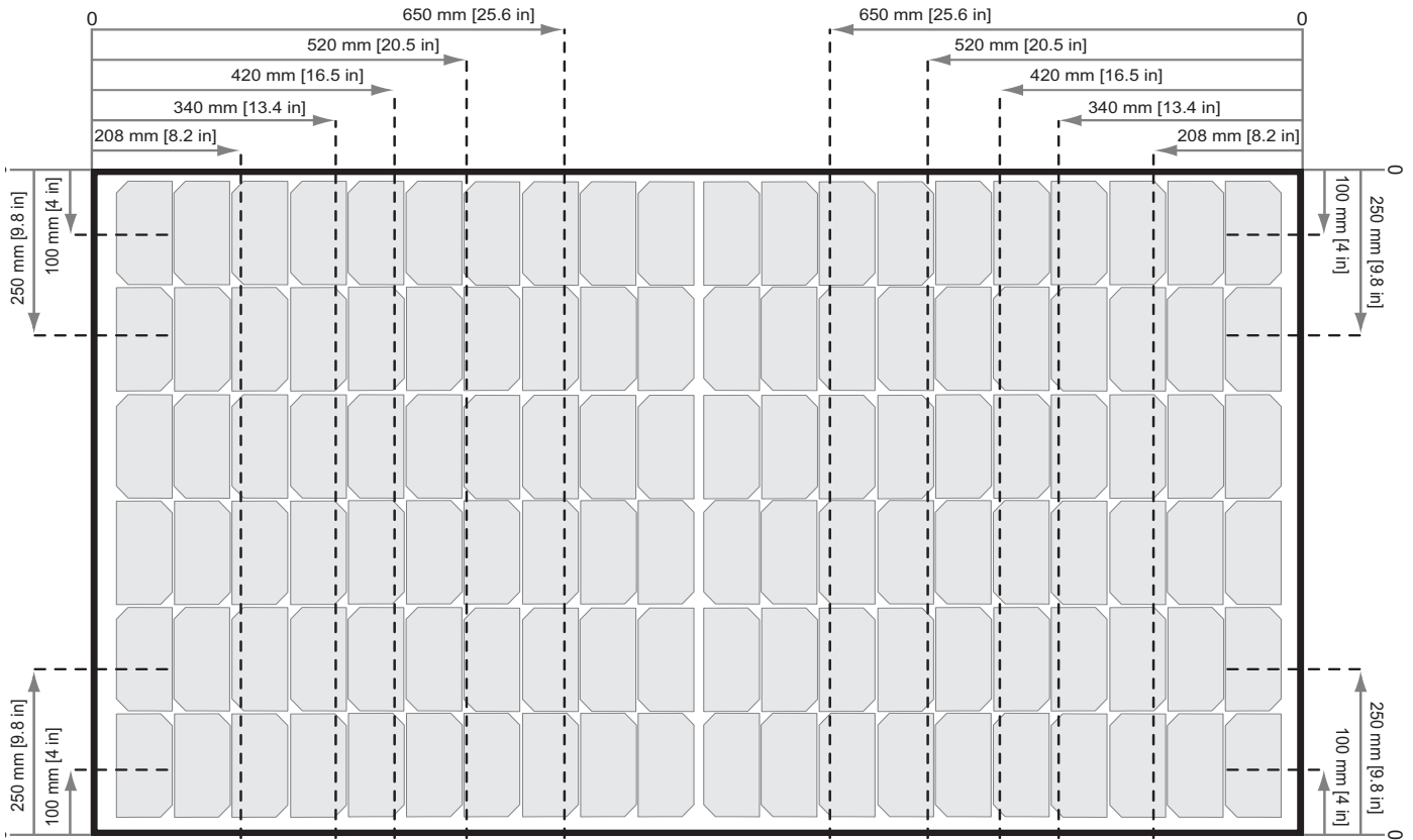
Fig. 6: Clamping of N-Peak panels on rails parallel to short side of module
