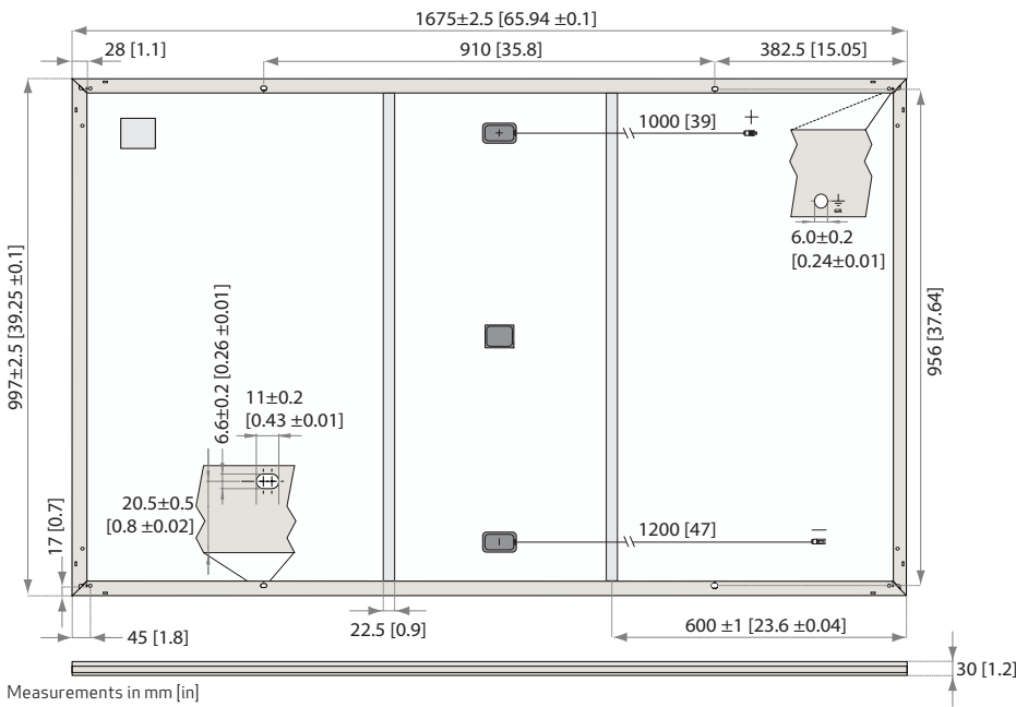
Fig. 22: Panel dimensions: REC N-Peak Series
