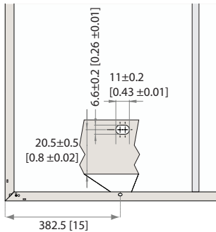
Fig. 12: Mounting holes: REC 60-cell panels
