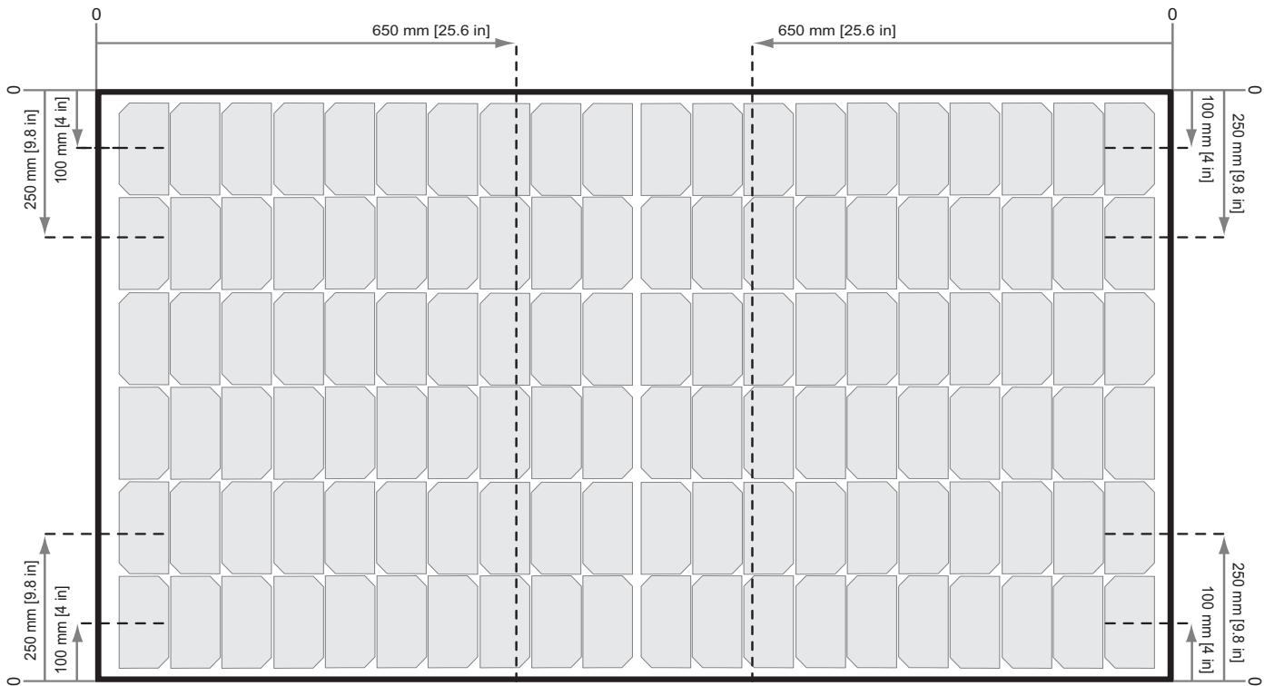
Fig. 7: Clamping of N-Peak panels on rails parallel to long side of module
