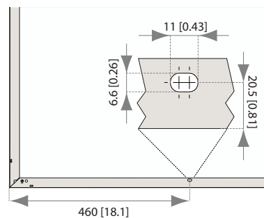
Fig. 13: Mounting holes: REC 72-cell panels
