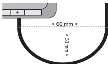
Fig. 18: Minimum cable bend radius
