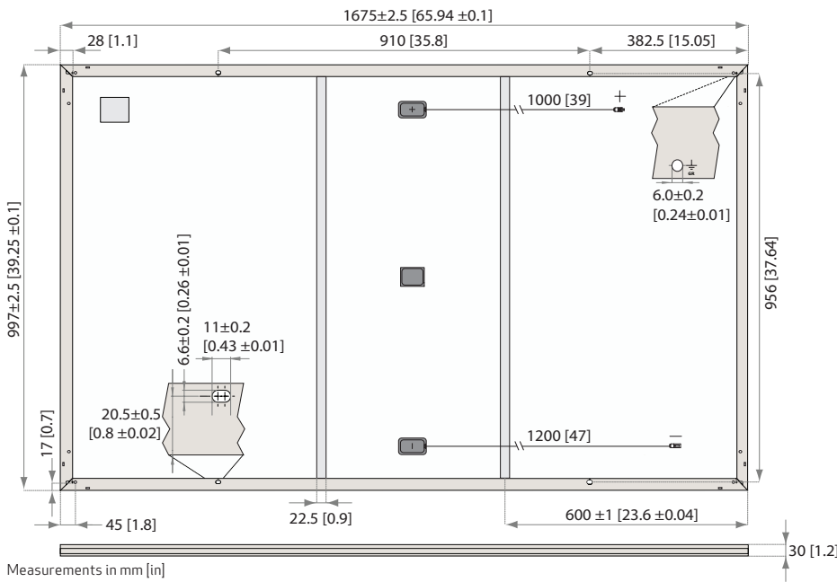
Fig. 23: Panel dimensions: REC N-Peak Black Series
