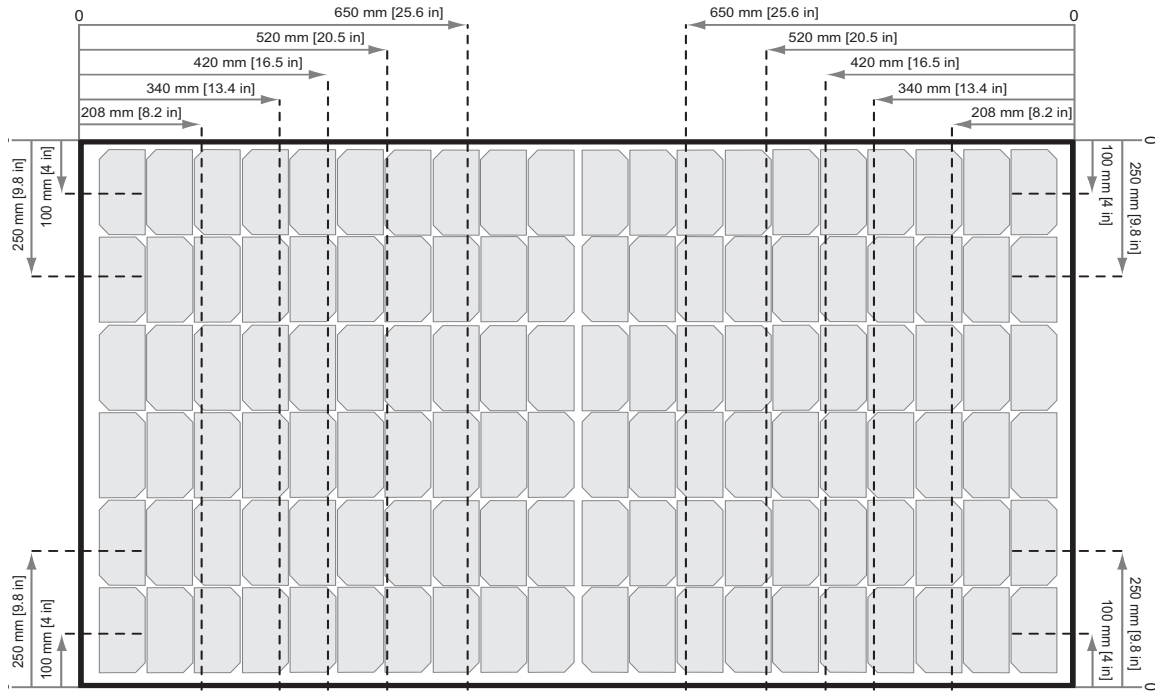
Fig. 8: Clamping of REC N-Peak Series panels using short rails
