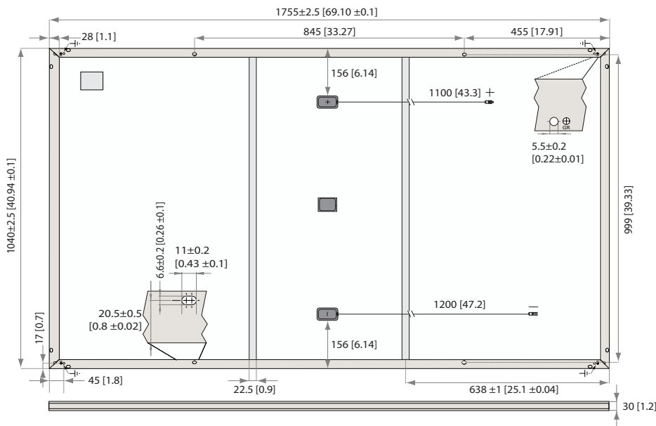
Fig. 20: Panel dimensions: REC TwinPeak4 Series
